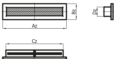
Shield grate / air intake KRCZNP 300x50
