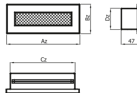
Shield grate / air intake KRCZNP 150x50, 200x50 and 200x90
