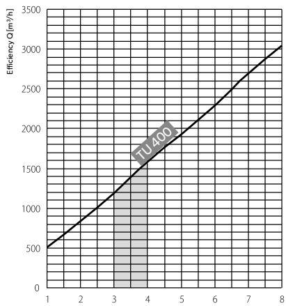
Efficiency chart for Turbowents (various diameters) in a function of wind speed, not including the influence of chimney height. (l[m/s]=3.6[km/h])
